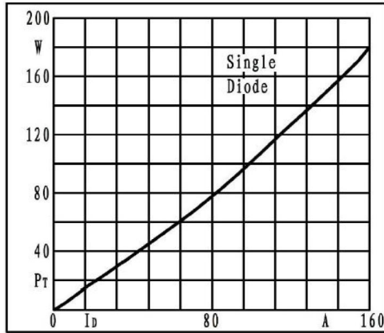
Fig2. Power dissipation
